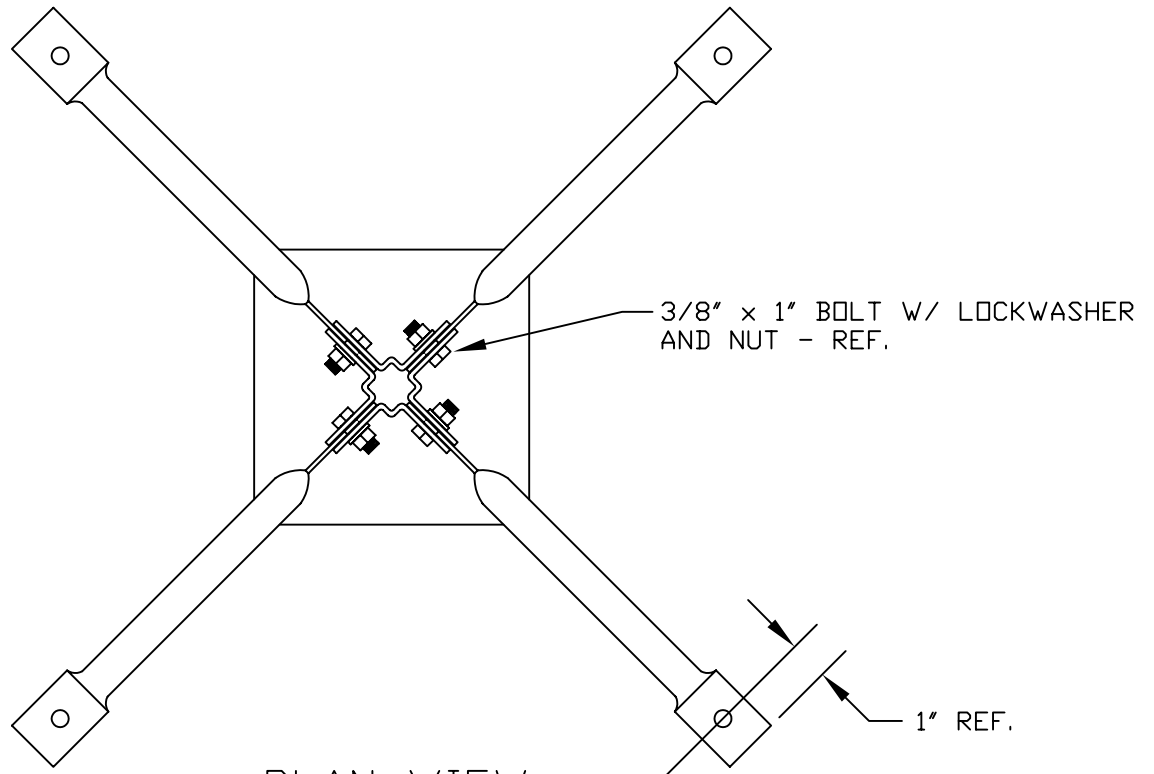
PLAN VIEW PEDESTAL HEAD ASSY. NOT SHOWN FOR CLARITY
