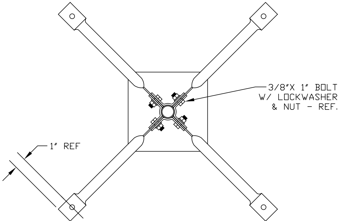
PLAN VIEW PEDESTAL HEAD ASSY. NOT SHOWN FOR CLARITY
