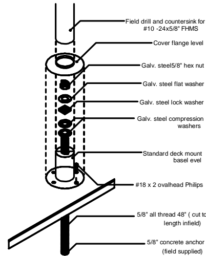
POST MOUNT AT ACCESS FLOOR
