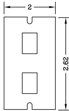
Part No. CAN12102 Device Plate For Mod. Jack Couplers
