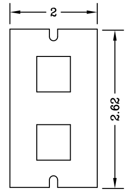
Part No. CAN12105 Device Plate For Lucent Univ. Collars
